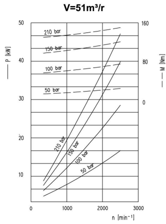
3.5系列功率性能曲线表/Group 3.5 Power Performance Curve Table
