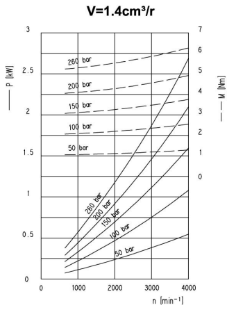
1.25系列功率性能曲线表/Group 1.25 Power Performance Curve Table
