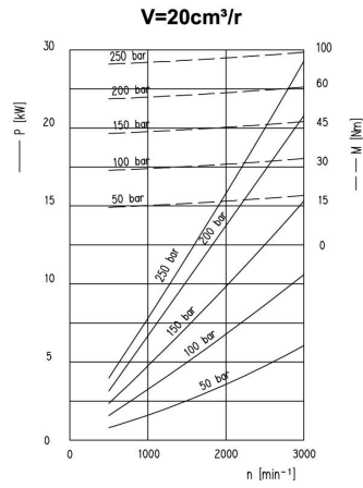
2系列功率性能曲线表/Group 2 Power Performance Curve Table
